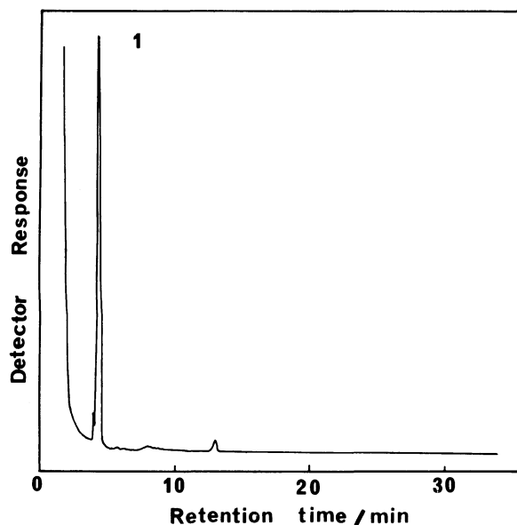
Fig. 2. The gas chromatogram of the TMS derivative of reduced product obtained by \gamma -irradiation in the presence of molecular sieves at 4 °C.
